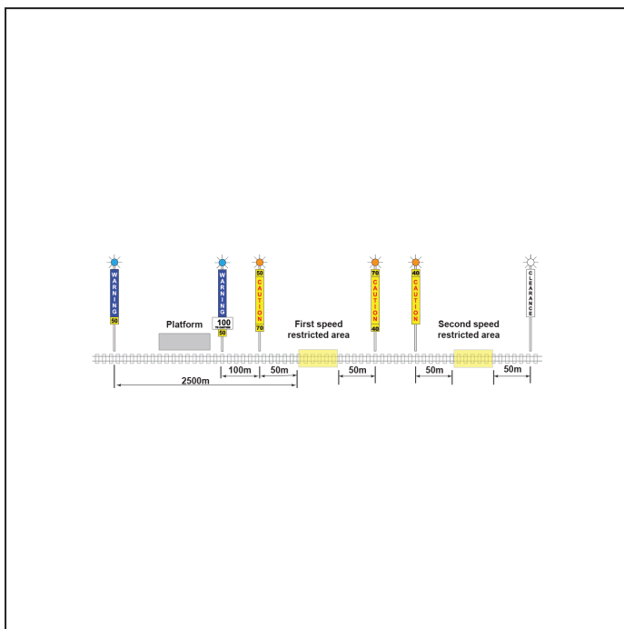
FIGURE 5: Placement of temporary speed signs where a platform is located before a multiple speed restricted area.
