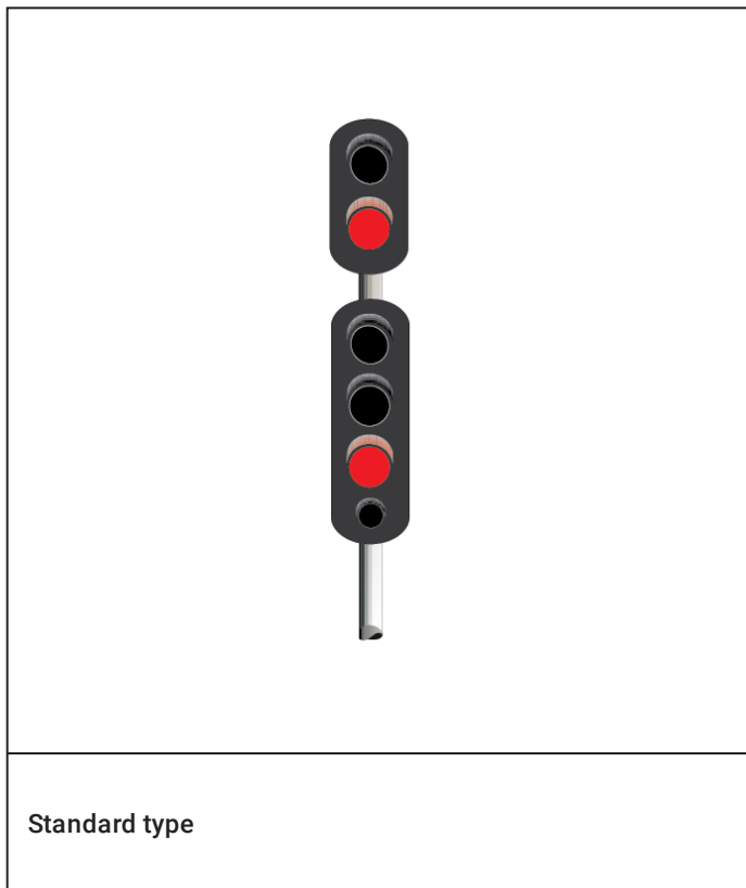
FIGURE 7: Vertical colour light forms
