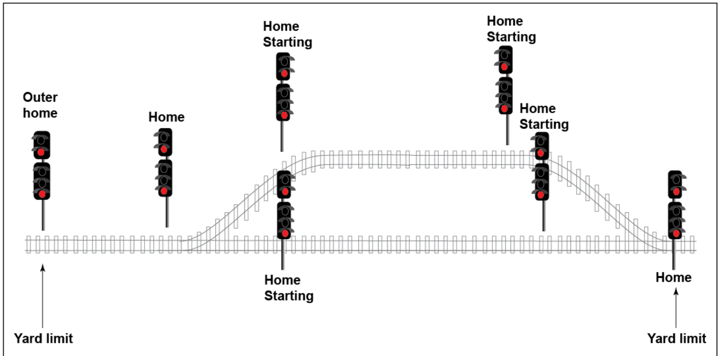
FIGURE 2: Example of yard limits in bidirectional single-line RVD territory.
