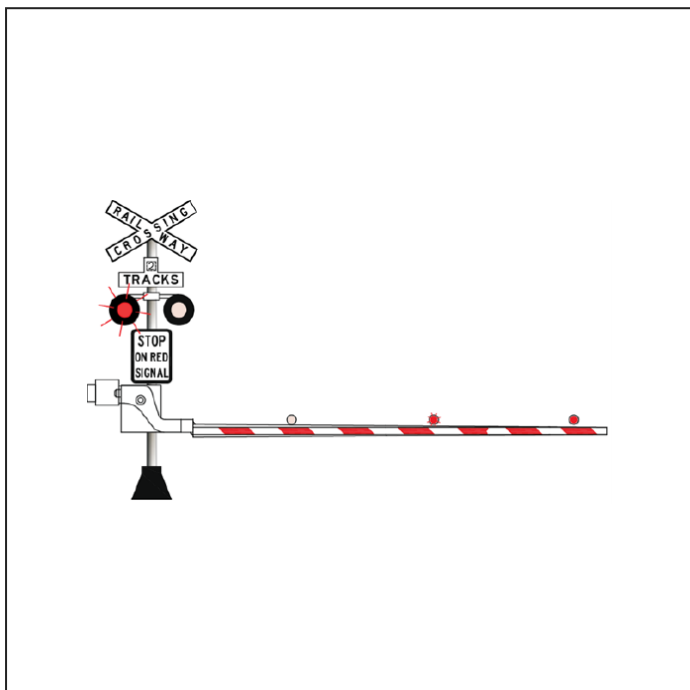
Figure 6: Examples of Type F roadside warning equipment with booms and lights
