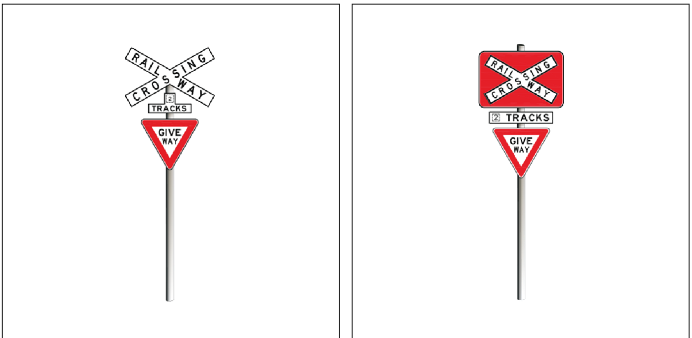
Figure 7: Examples of Type B level crossing GIVE WAY signs
