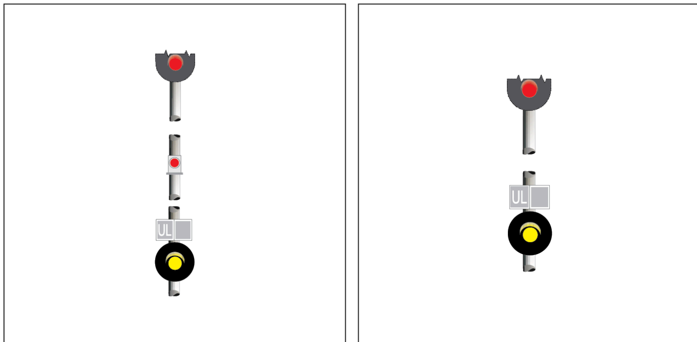
FIGURE 2: Examples of colour light shunting signals displaying PROCEED.
