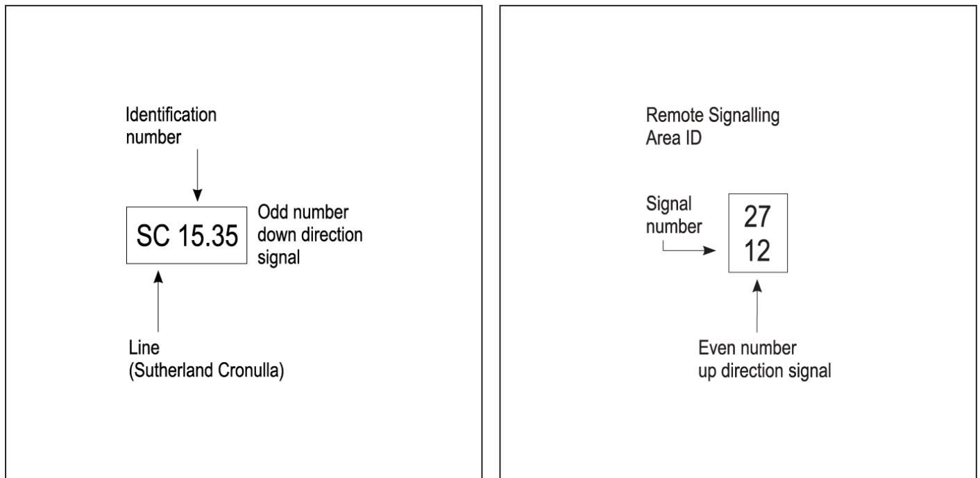
FIGURE 43: Examples of signal identification signs.
