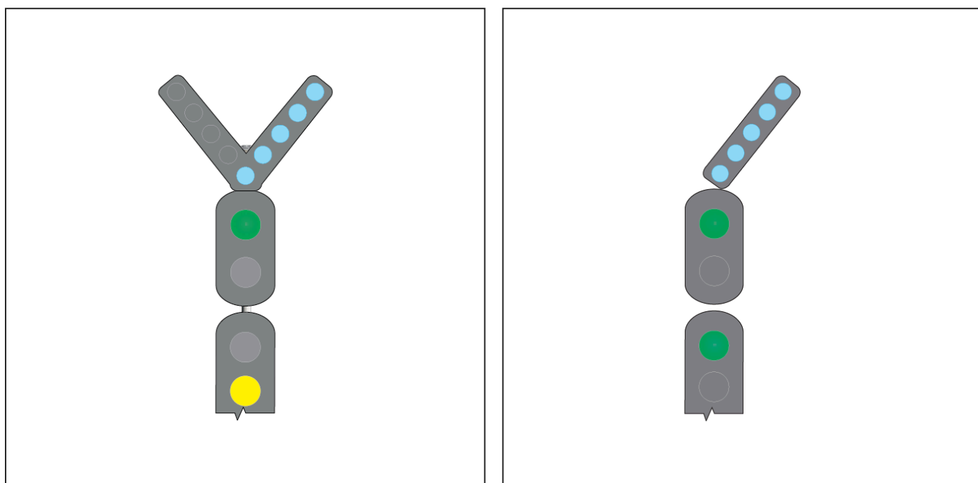
FIGURE 10: Examples of turnout repeaters.
