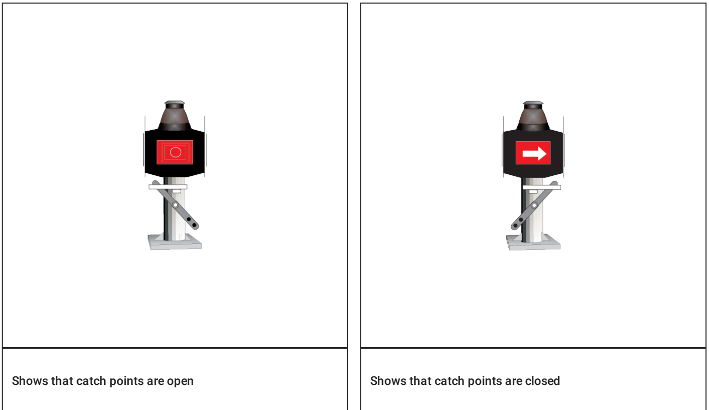
FIGURE 6: Examples of arrow type mechanical catch point indicators.
