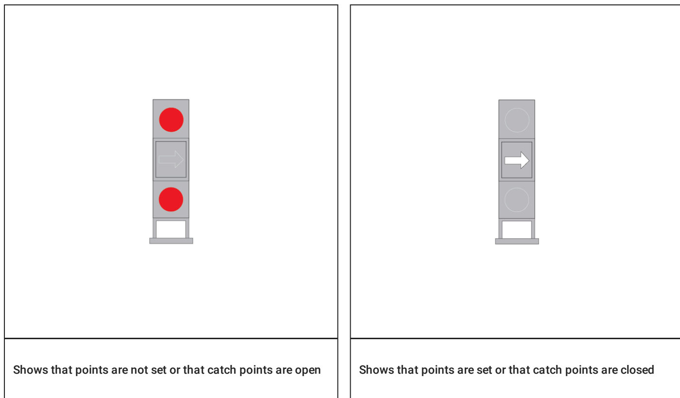
FIGURE 4: Example of vertical colour light trailing point or catch point indicators.
