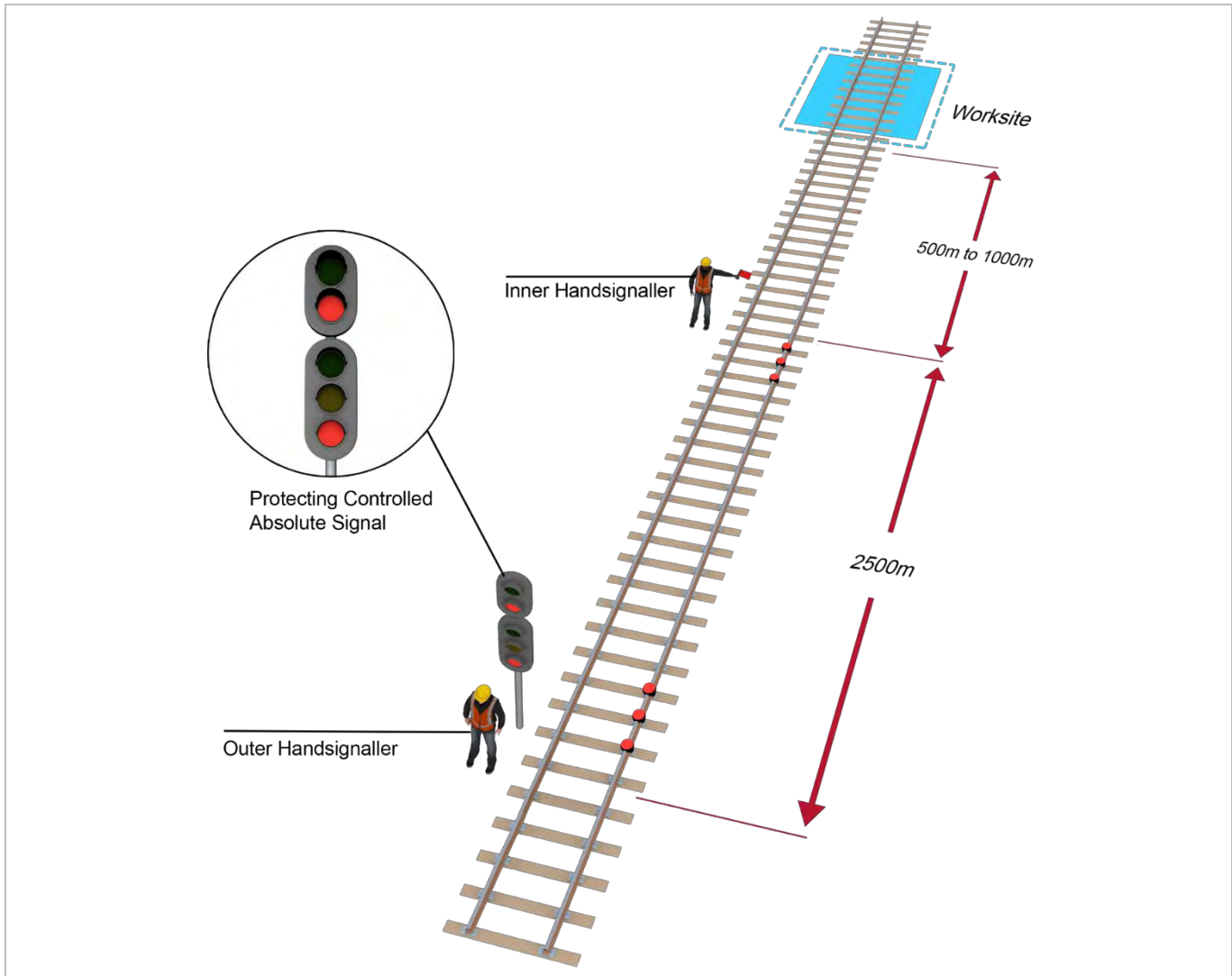
FIGURE 5: Example of protecting a worksite with a controlled absolute signal more than 1000m and less than 3500m from the worksite.
