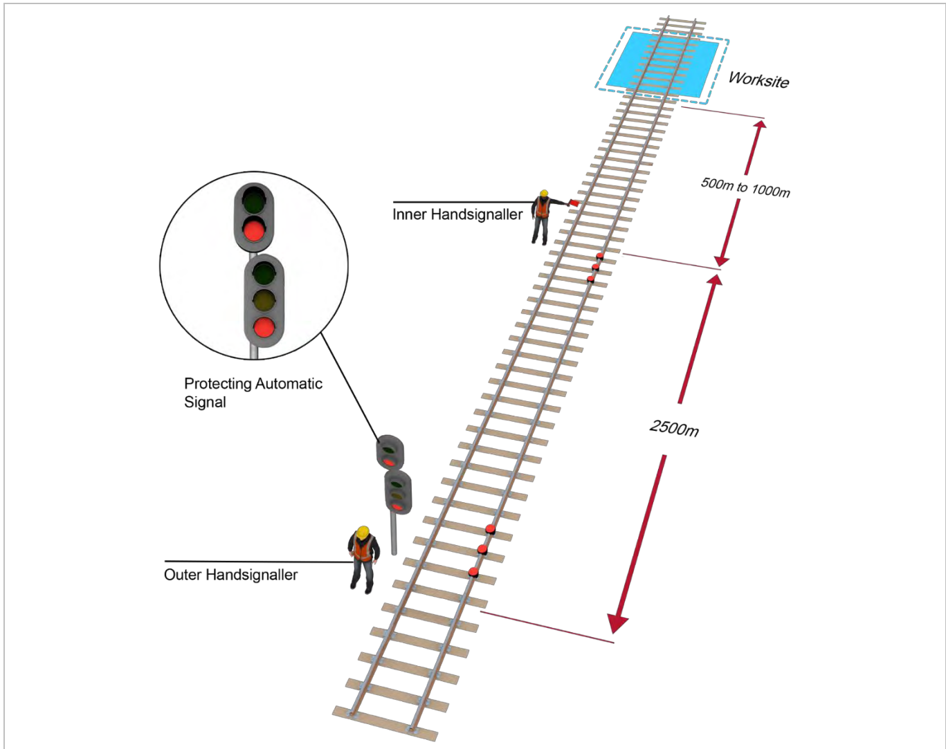
FIGURE 6: Example of protecting a worksite with an automatic signal more than 1000m and less than 3500m from the worksite.
