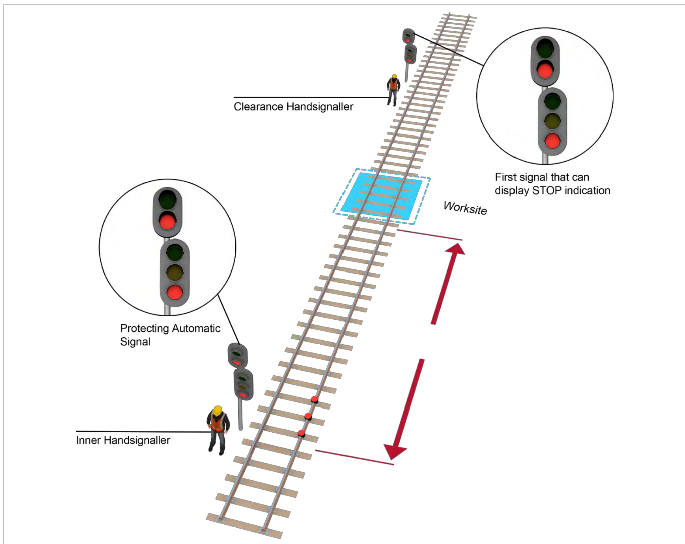
FIGURE 13: Example of placement of a clearance Handsignaller at the first signal that can display a STOP indication, to tell the Protection Officer when the line is clear for rail traffic to approach.
