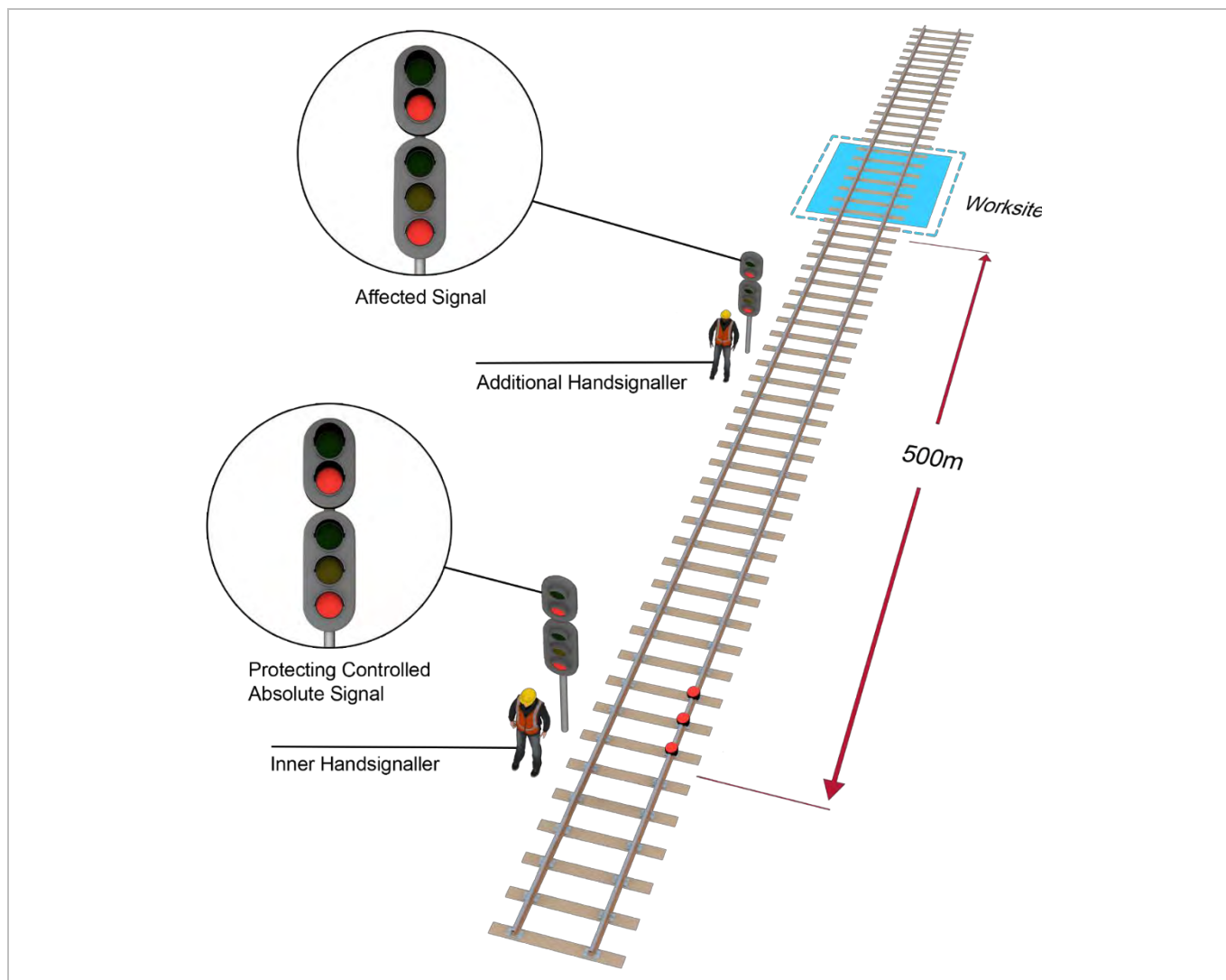
FIGURE 8: Example of additional Handsignaller placed when the signal between the worksite and the protecting signal cannot be cleared.
