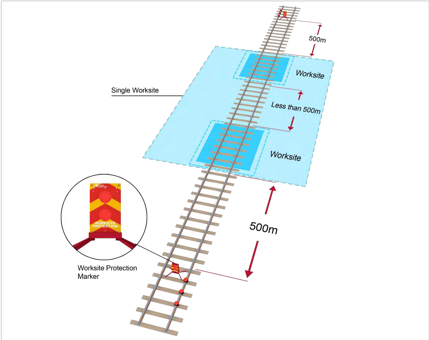
FIGURE 5: Example of protection arrangements for worksites less than 500m apart protected as a single worksite.
