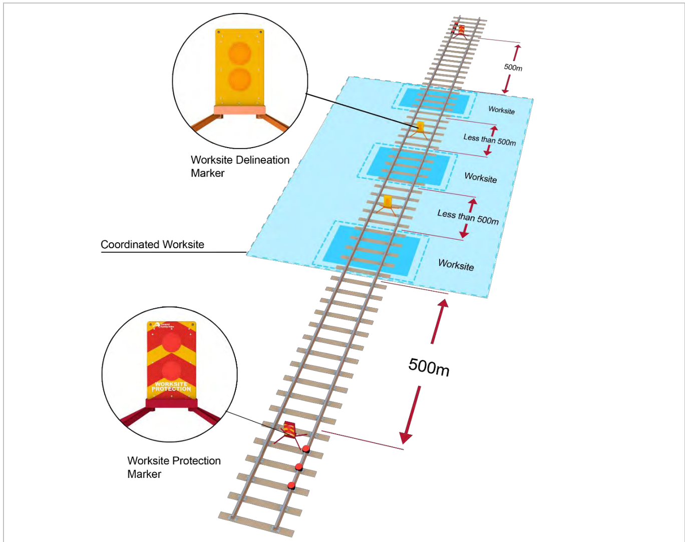
FIGURE 6: Example of protection arrangements for worksites less than 500m apart protected as a coordinated worksite.
