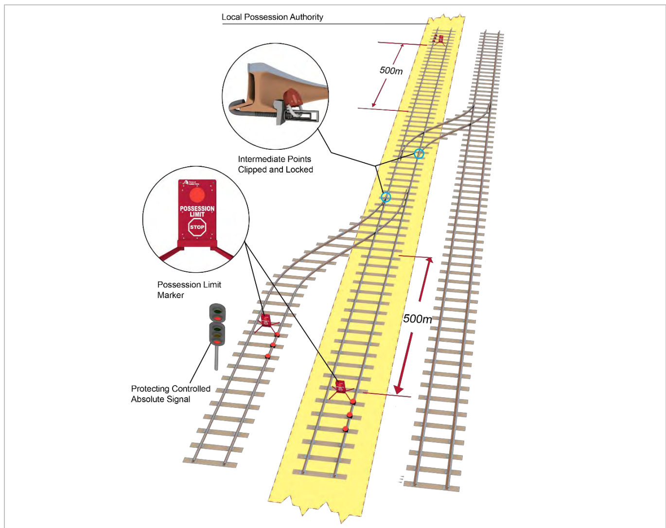
FIGURE 7: Example of protection arrangements if rail traffic is authorised to cross the LPA area.
