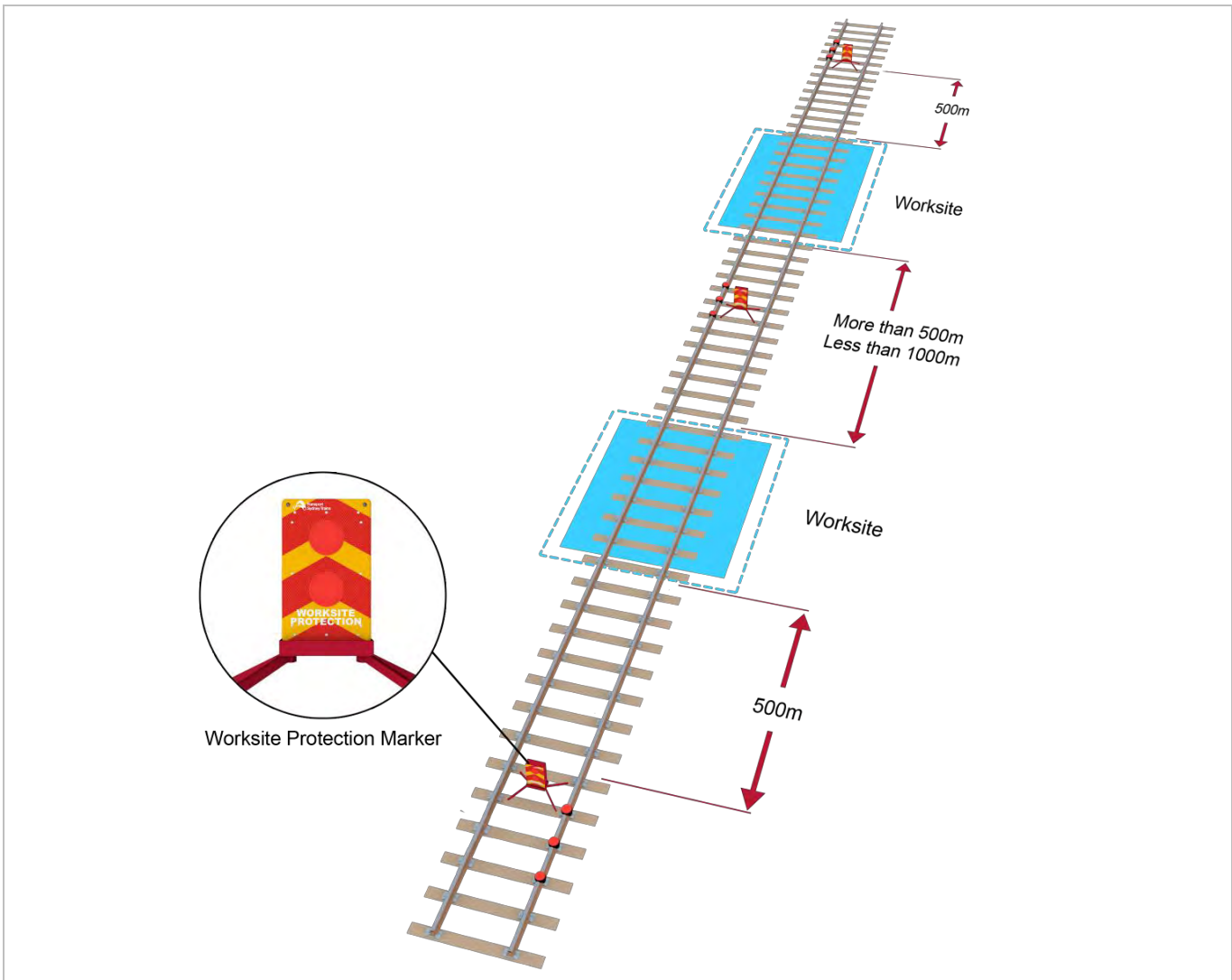
FIGURE 4: Example of protection arrangements for multiple worksites between 500m and 1000m apart
