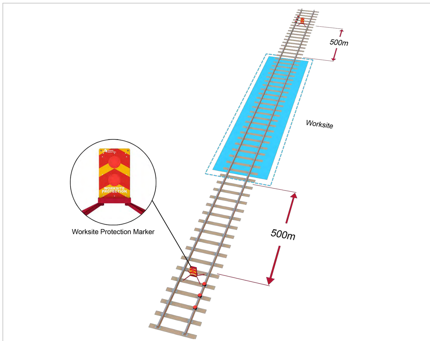
FIGURE 3: Example of protection arrangements for a single worksite
