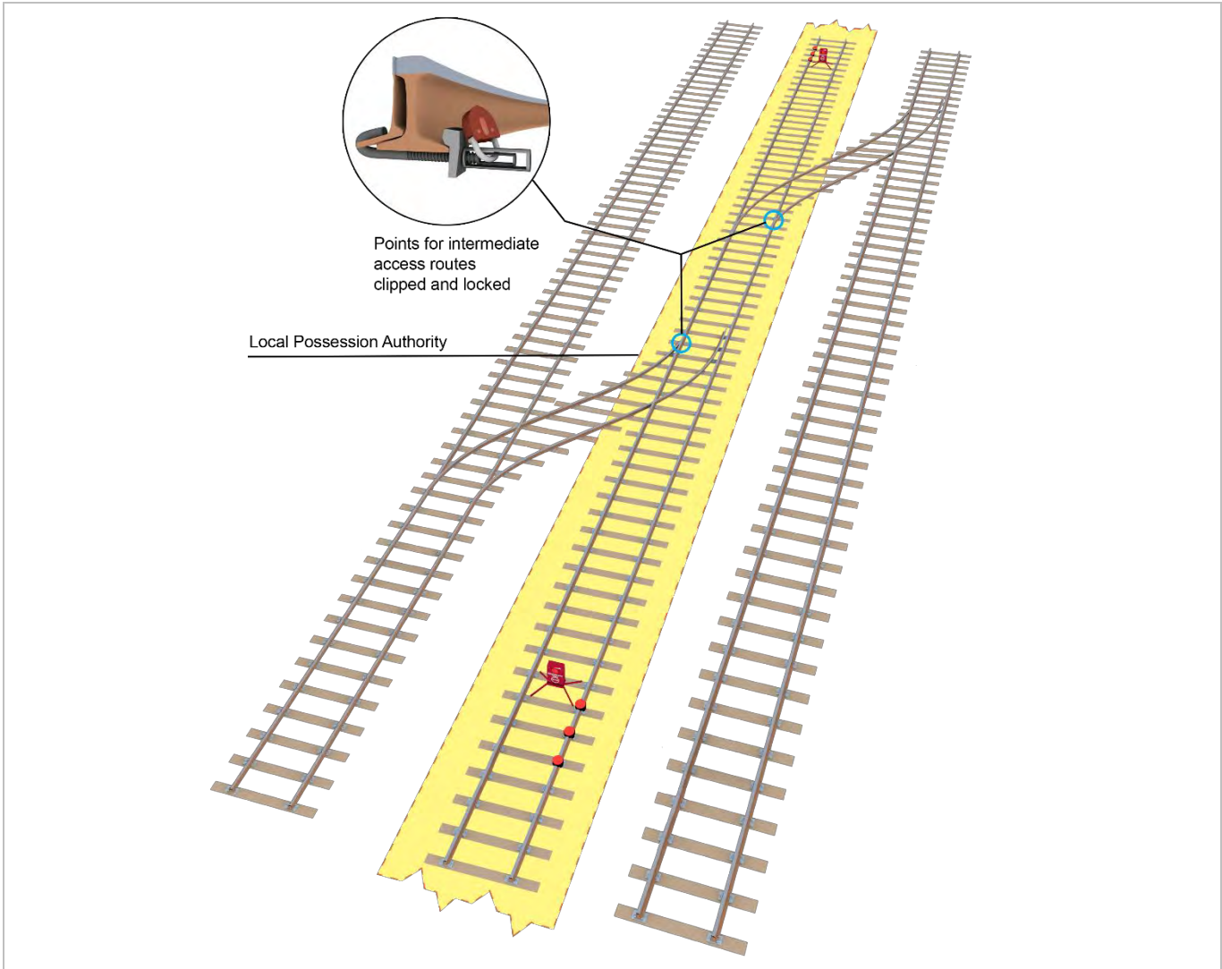
FIGURE 2: Example of points for intermediate access routes clipped and locked
