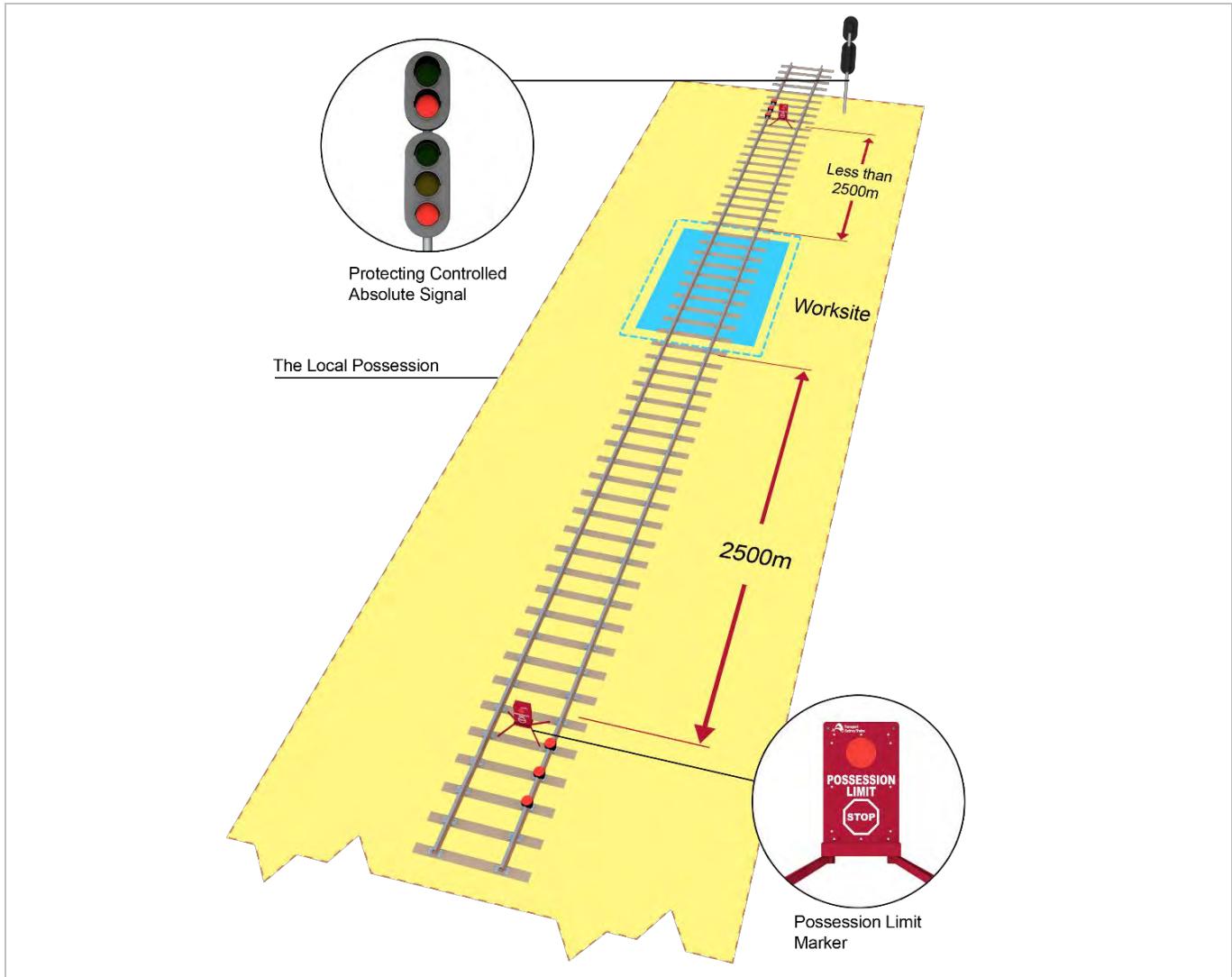
FIGURE 1: Example of protection arrangements for an LPA
