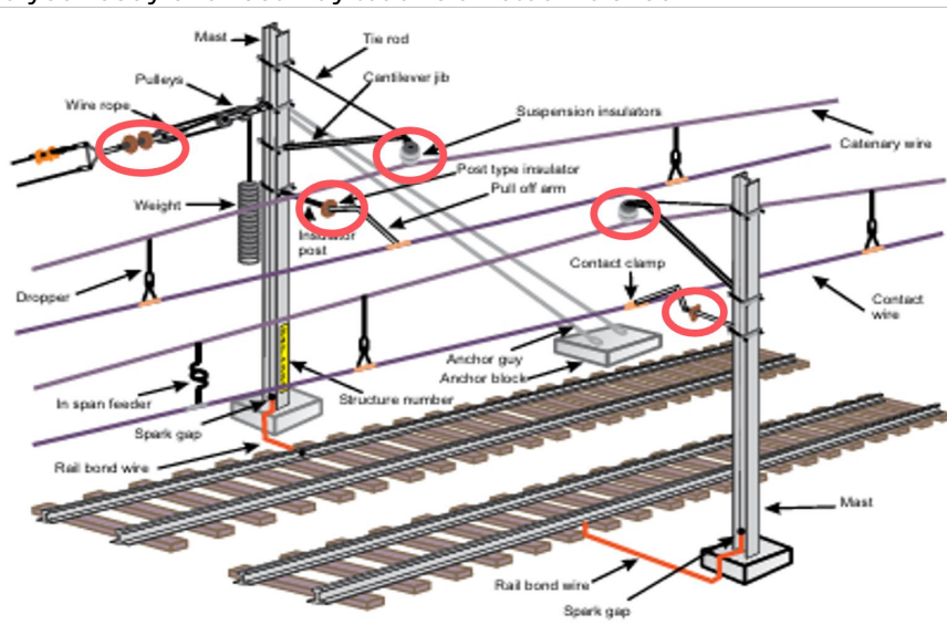
Figure 1 - OHW structures equipped with a spark gap prevent the structure from remaining live at 1500 V d.c. in the event of a faulty insulator (circled).
