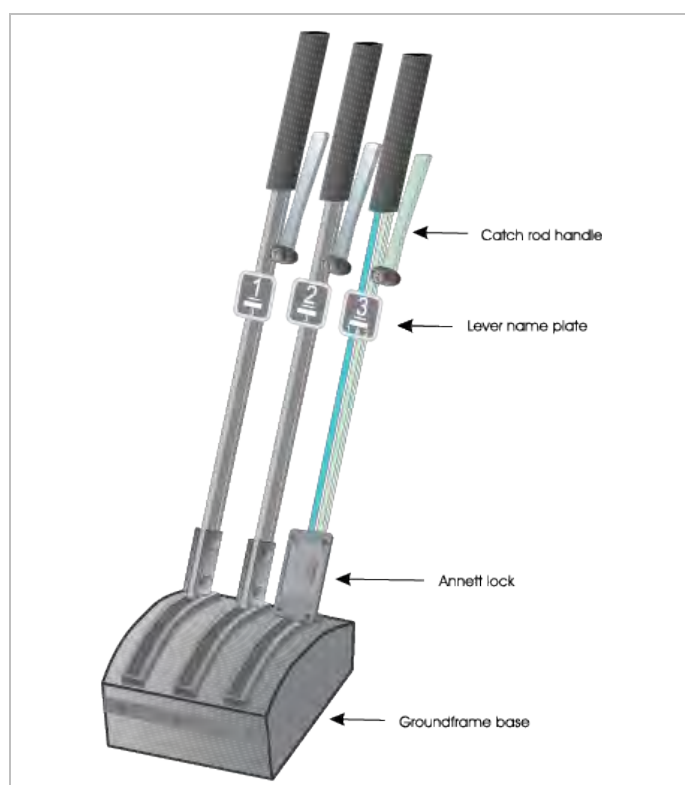
FIGURE 1: FIGURE 1: Groundframe.
