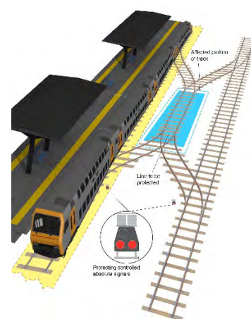
FIGURE 1: Example of protecting the affected portion of track when it is not required to protect the full length of rail traffic.
