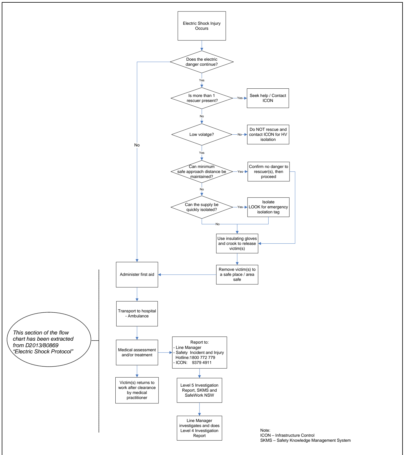
Figure 2 Release and rescue procedure in the event of a live LV electrical accident
