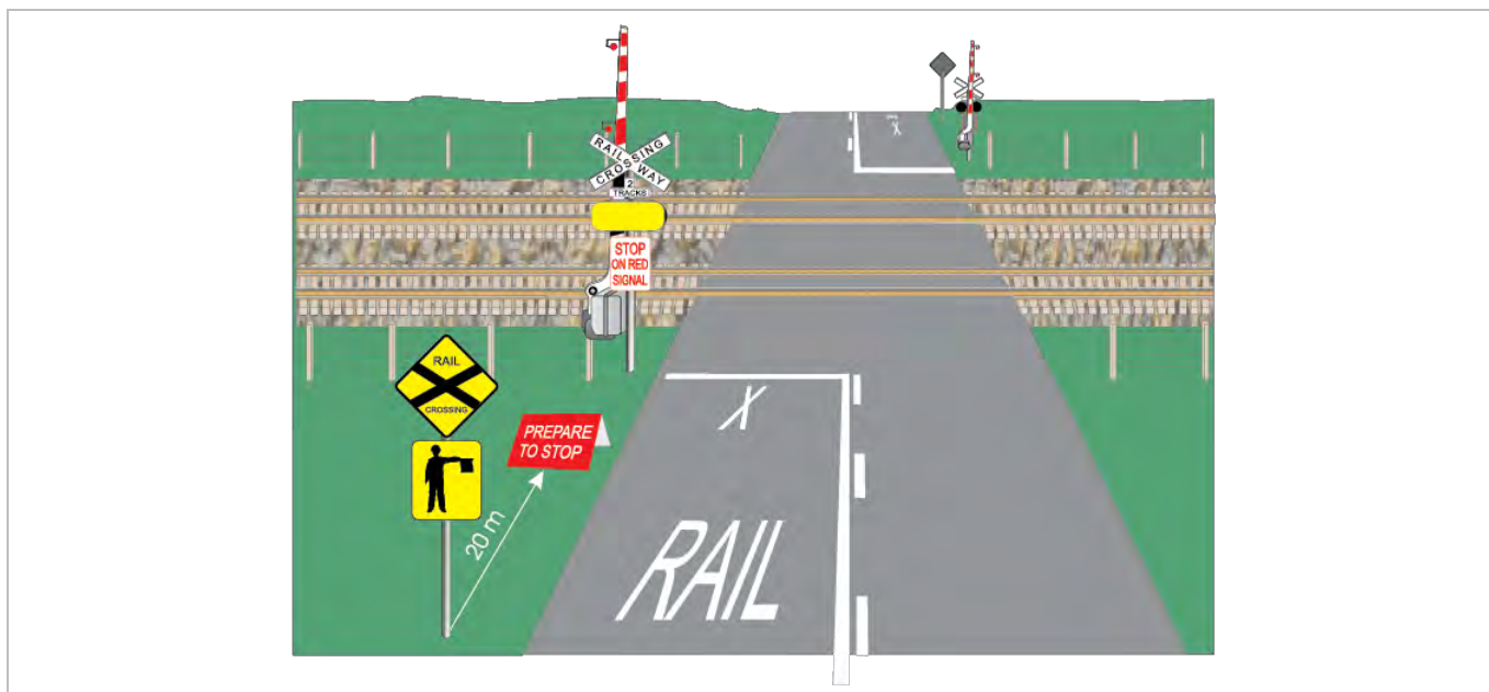
FIGURE 1: Emergency roadside warning equipment applied to Type F level crossing warning equipment.
