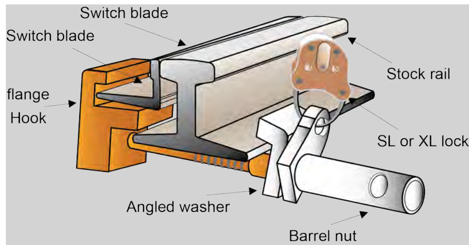
FIGURE 3: Example of a fitted tangential point clip
