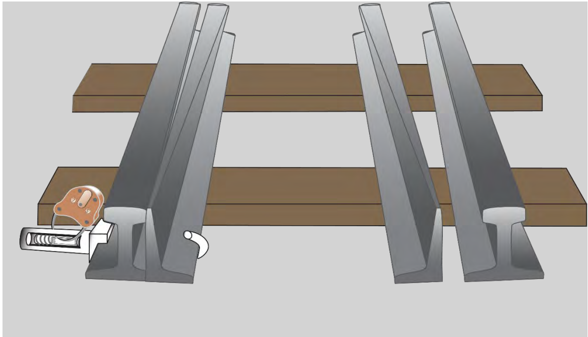
FIGURE 4: Example of point clip fitted as close as possible to tapered end of a switch blade.
