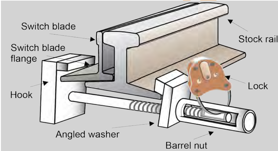
FIGURE 2: Example of a fitted Conventional point clip
