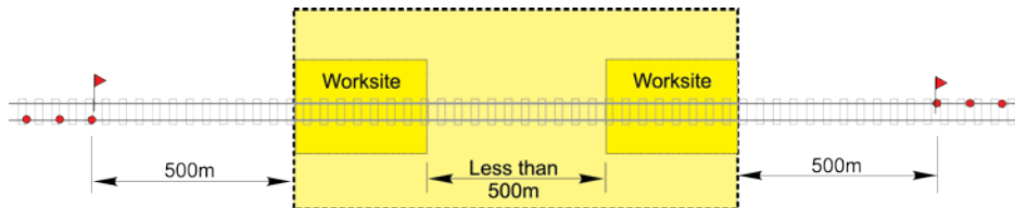
FIGURE 4: Example of protection arrangements for worksites less than 500m apart protected as a single worksite.
