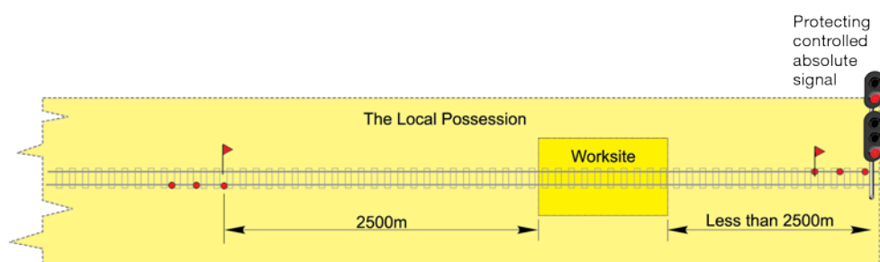
FIGURE 1: Example of protection arrangements for an LPA
