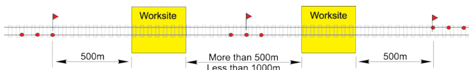
FIGURE 3: Example of protection arrangements for multiple worksites between 500m and 1000m apart
