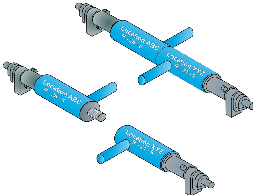
FIGURE 1: Half pilot staffs - separated and joined
