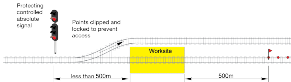
FIGURE 3: Example of protecting signal less than 500m from worksite, with points clipped and locked for a different route
