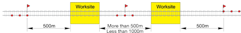
FIGURE 5: Example of protection arrangements for multiple worksites between 500m and 1000m apart
