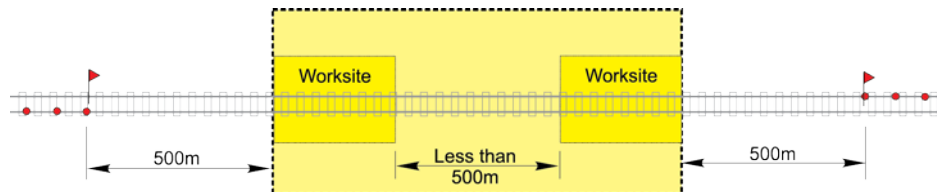
FIGURE 6: Example of protection arrangements for worksites less than 500m apart protected as a single worksite.
