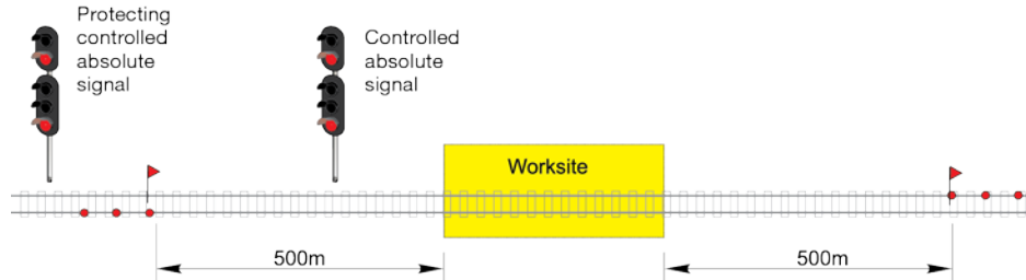
FIGURE 2: Example of protection arrangements for a worksite when the closest signal is less than 500m from the worksite, a signal more than 500m from worksite must be used for protection
