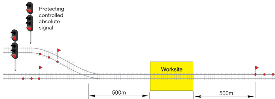
FIGURE 4: Example of protecting a worksite with signals more than 500m from worksite
