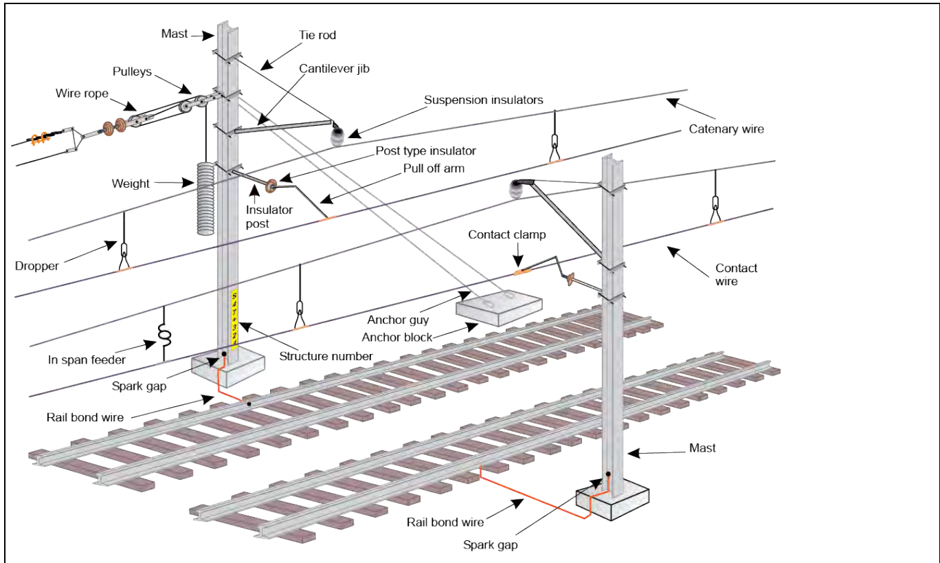
FIGURE 2: Simple catenary, regulated-tension, cantilever construction on masts
