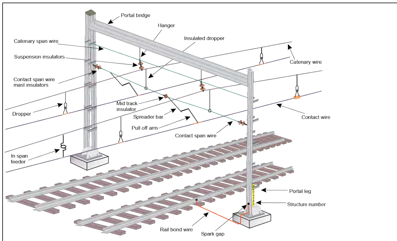
FIGURE 1: Simple catenary, fixed-anchored, span-wire construction on portal structures
