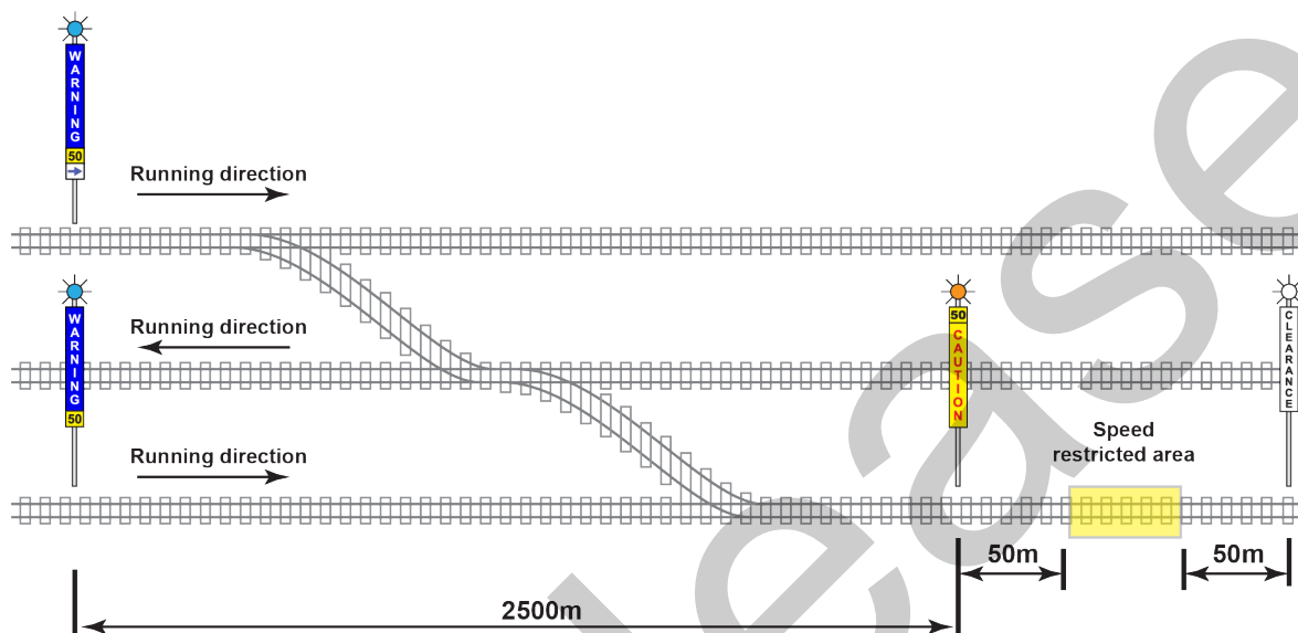
FIGURE 6: Location of temporary speed signs for speed restricted area with multiple routes
