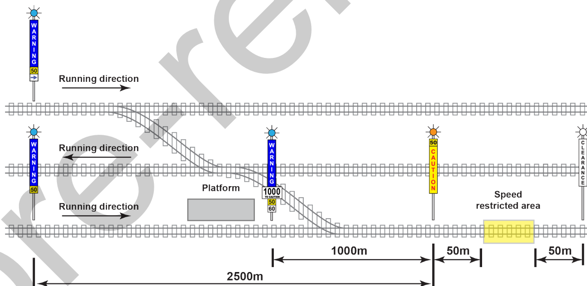
FIGURE 7: Location of temporary speed signs where a platform is located before a multiple route speed restricted area
