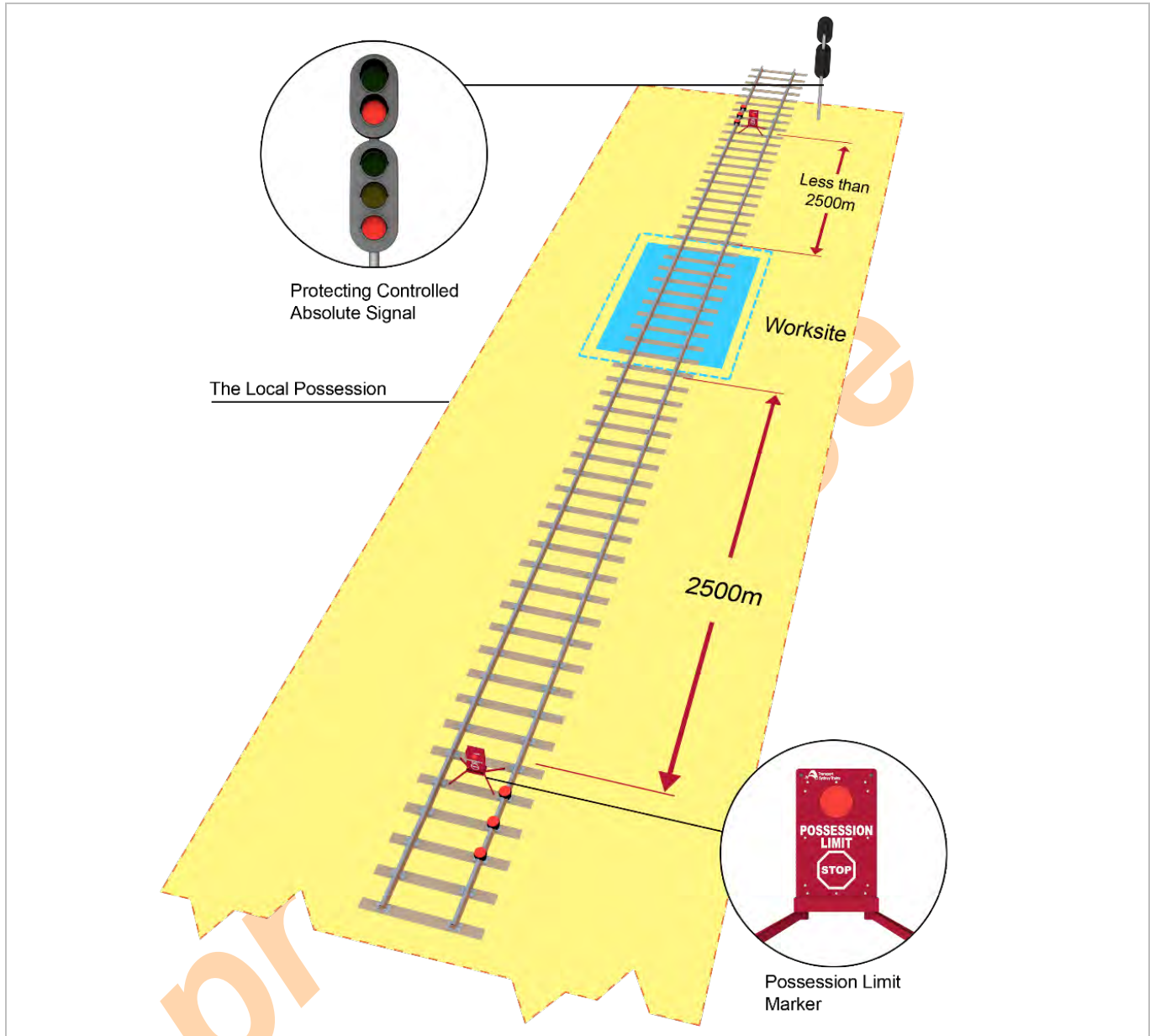
FIGURE 1: Example of protection arrangements for an LPA
